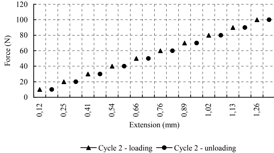
Figure 6: Flexural test of the sandwich panel clamped on contour. Cycle 2 loading-unloading
