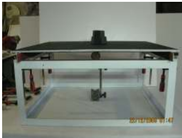
Figure 3: Three-point bend load-unload test detail. Sandwich panel supported linearly on two opposite edges
