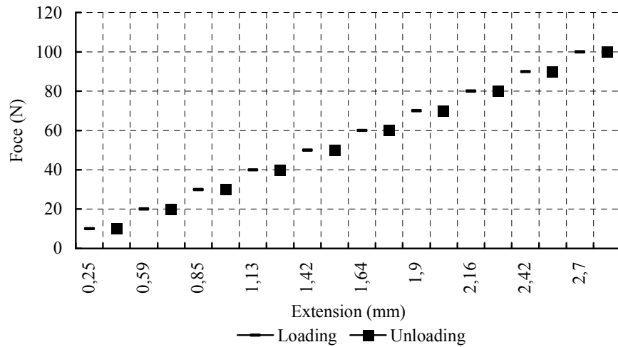
Figure 7: Three-point bend test of the sandwich panel supported linearly on two opposite edges
