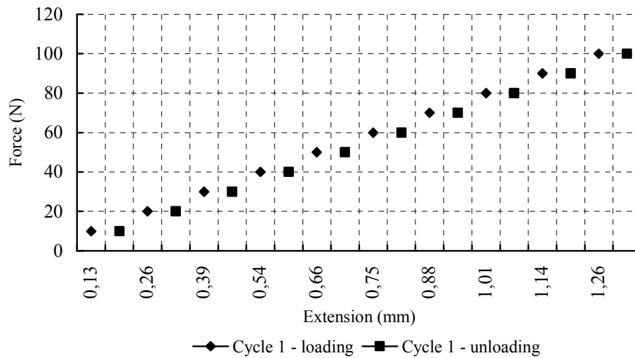
Figure 5: Flexural test of the sandwich panel clamped on contour. Cycle 1 loading-unloading
