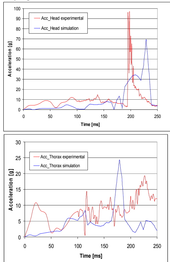
Fig. 18. Comparison between theoretical and experimental values
