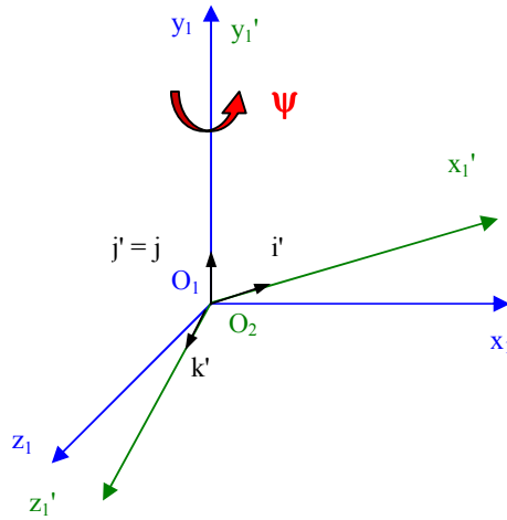
Fig. 4 Rotation with ψ angle
