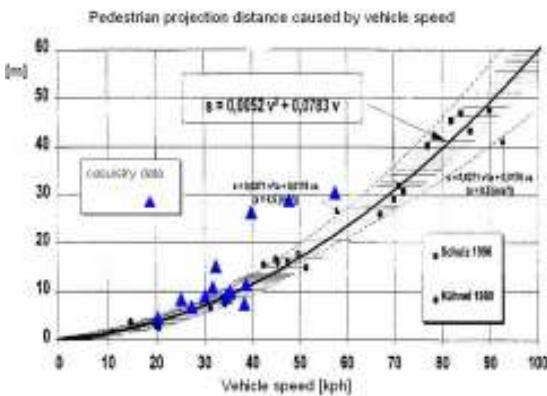
Fig. 17 Comparison between the Kuhnel-Schulz curve and authors studied casuistry
