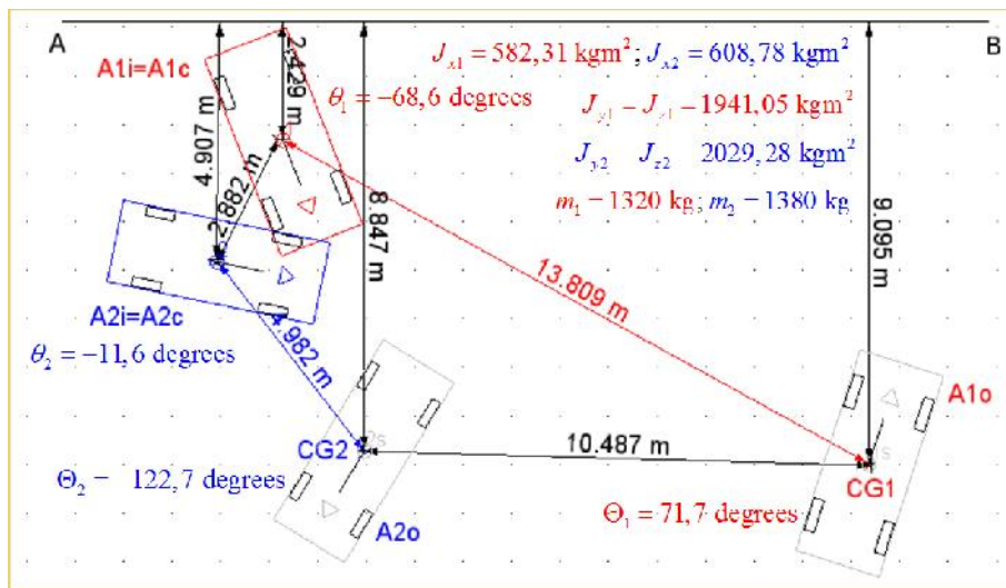
Figure 1: Car crash scene
