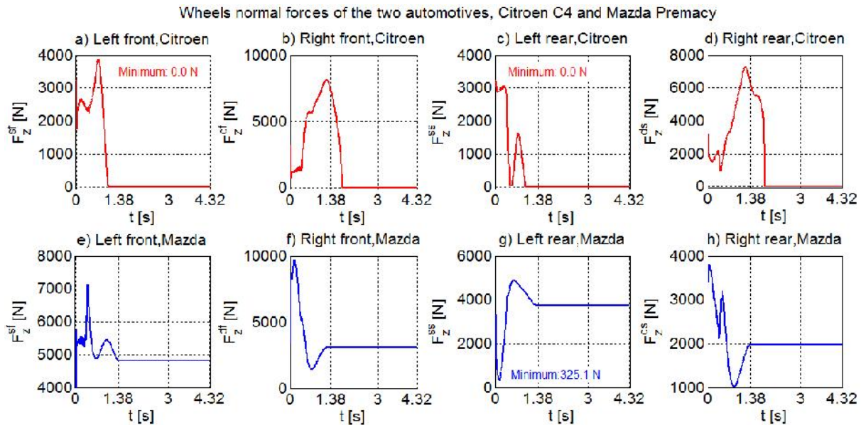
Figure 8: Normal forces to automotive wheels
