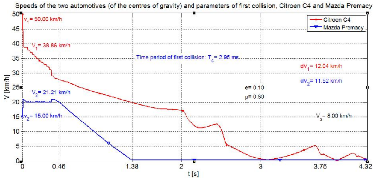
Figure 5: Automotive speeds (of centres of gravity)
