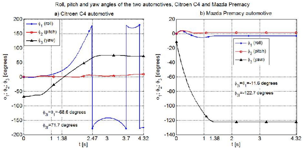
Figure 7: Rolling angles around coordinate axes
