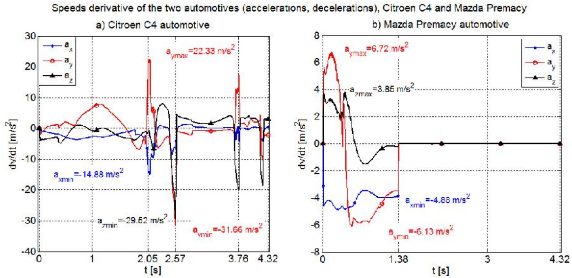
Figure 9: The derivative of automotive speeds (accelerations/decelerations centres of gravity)
