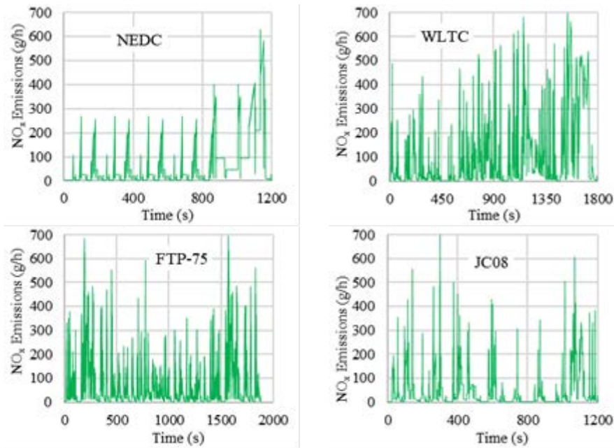
Fig. 6 – NO x emissions for the analyzed test cycles.
