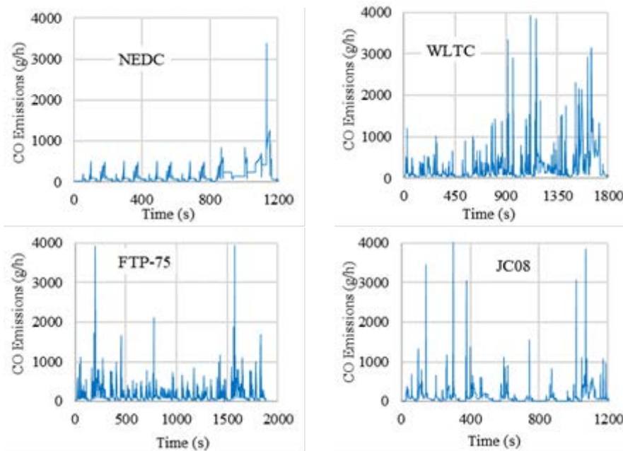
Fig. 7 – CO emissions for the analyzed test cycles.
