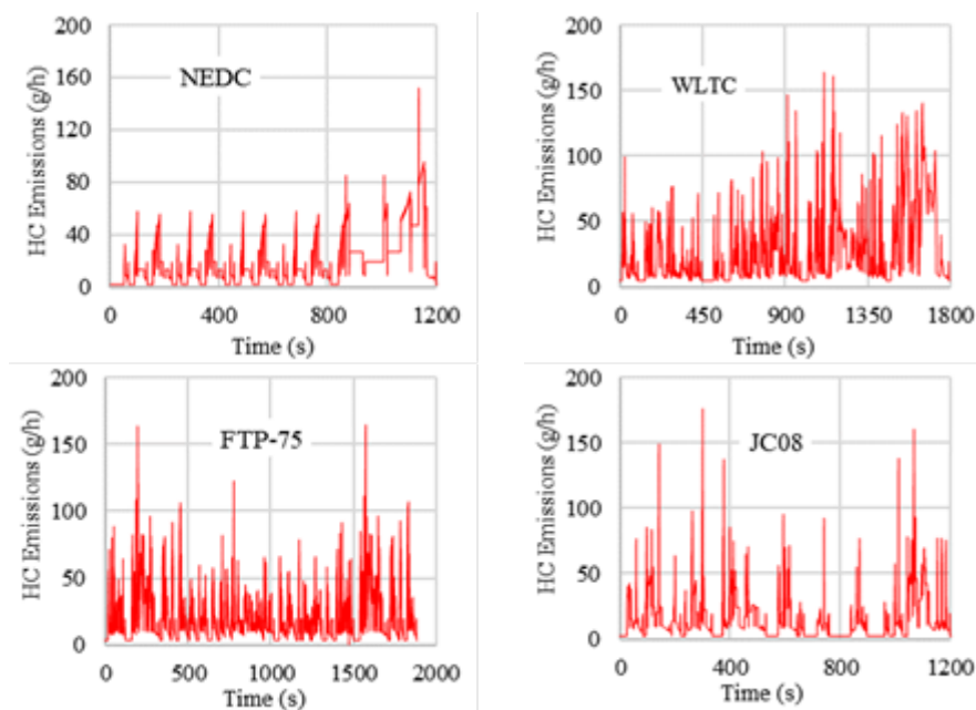
Fig. 8 – HC emissions for the analyzed test cycles.
