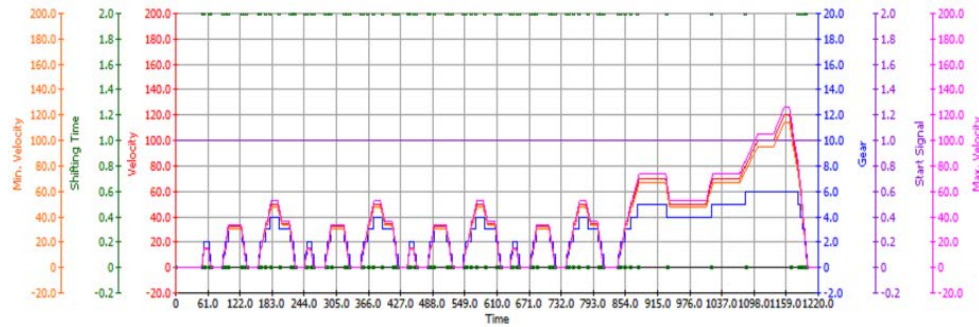
Fig.1 – NEDC Driving Cycle implemented in AVL Cruise.
