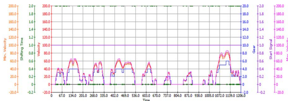
Fig. 4 – JC08 Driving Cycle.
