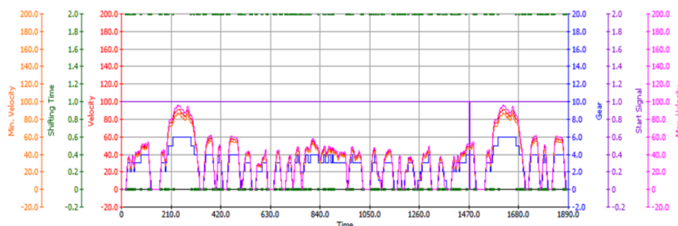
Fig. 3 – FTP-75 Driving Cycle implemented in AVL Cruise.
