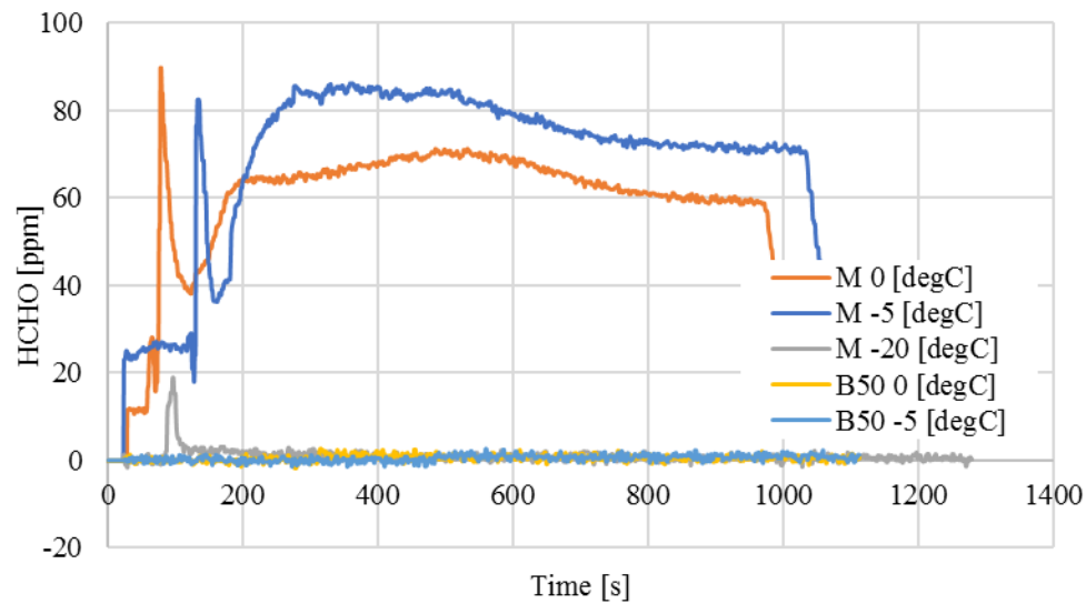
Fig. 9 – HCHO emissions for the five measurements [8].
