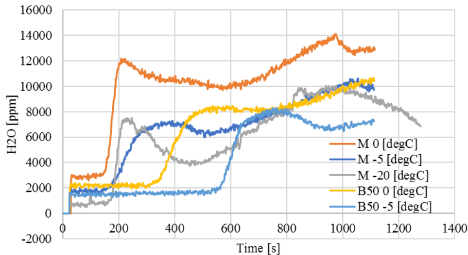
Fig. 8 – H 2 O emissions for the five measurements [8].
