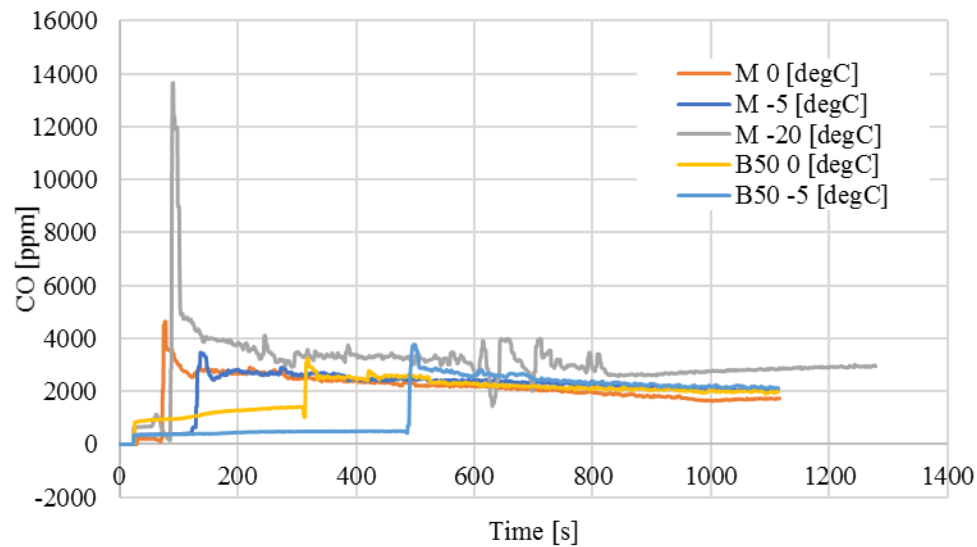
Fig. 10 – CO emissions for the five measurements [8].
