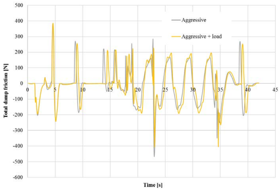
Fig. 15 – Total Damp Friction for the front left damper from IPG CarMaker for the loaded and unloaded vehicle with an aggressive driver.
