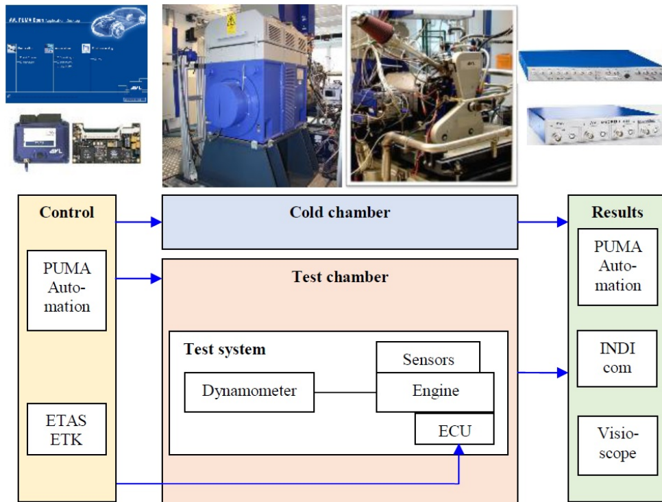
Fig. 1 – Information flow and control in the Laboratory.
