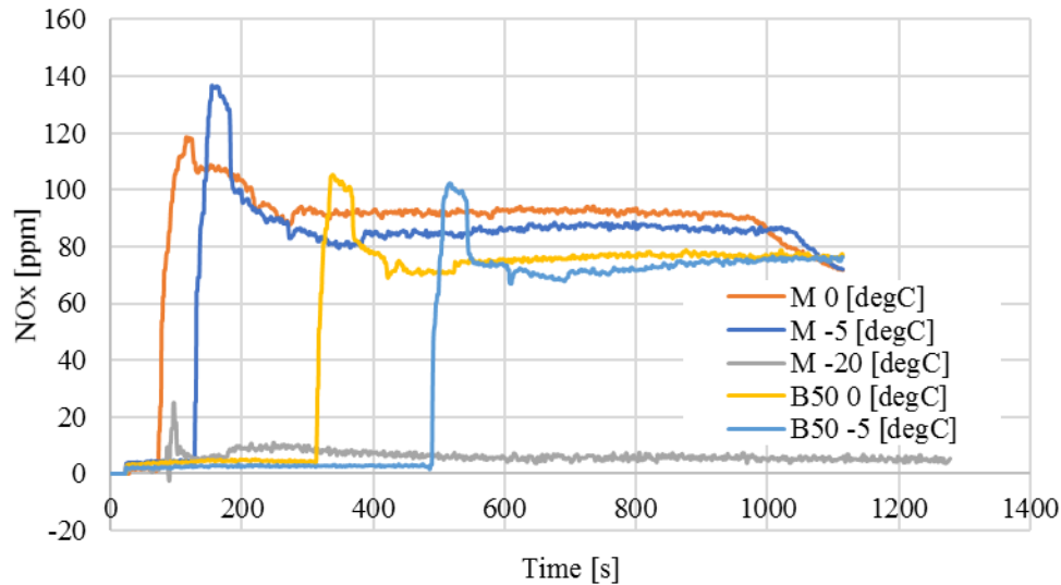
Fig. 11 – NO x emissions for the five measurements [8].
