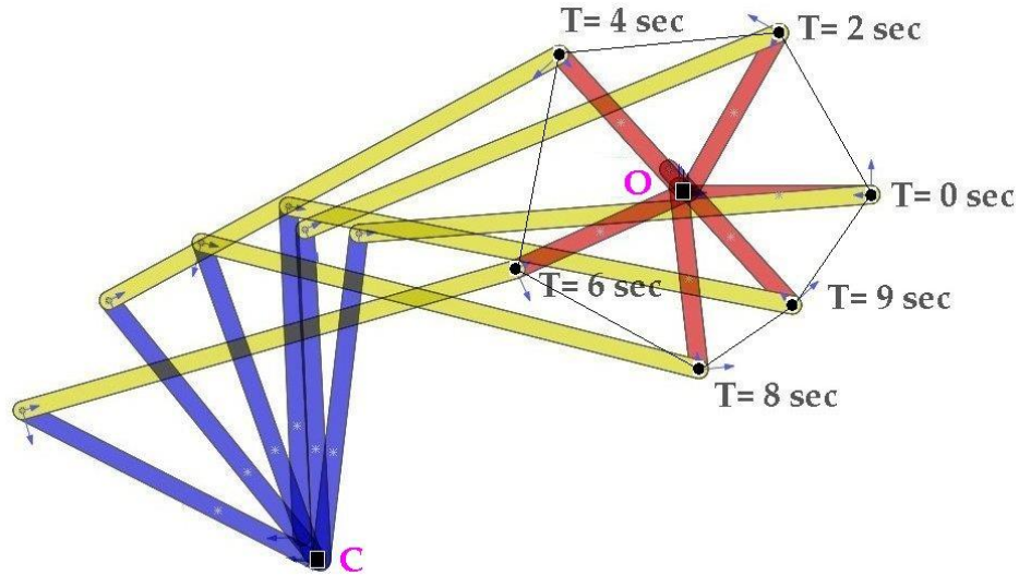
Figure 3: The successive positions of the quadrilateral mechanism
