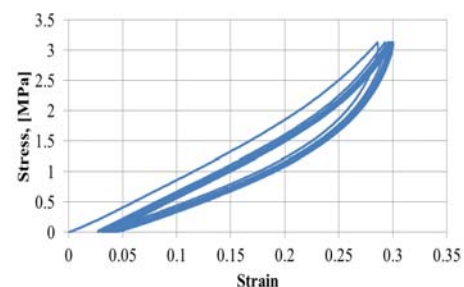
Fig. 4. The stress-strain curves of CR
