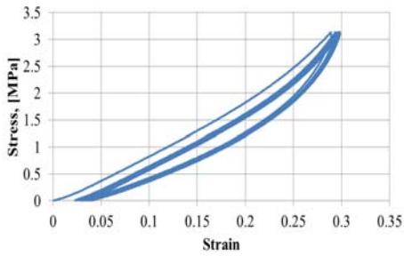
Fig. 5. The stress-strain curves of NR
