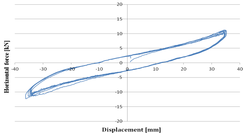
Fig. 12. The force-displacement curves of elastomeric bearings
