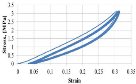
Fig. 7. The stress-strain curves of SBR
