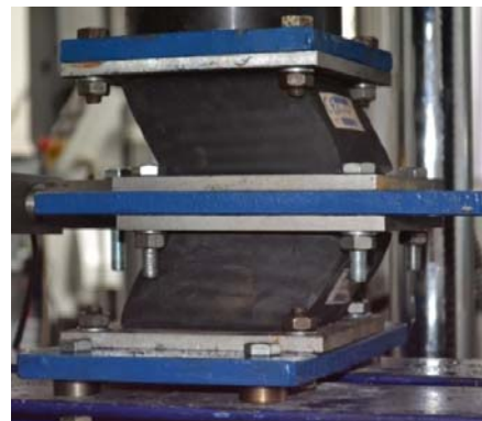
Fig. 11. The elastomeric bearing displacement
