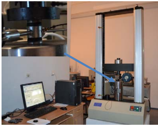
Fig. 9. The equipment for the dynamic test
