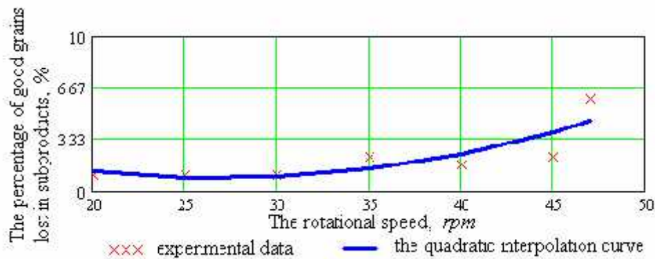
Figure 3: The variation of the percentage of good grains lost in subproducts depending on the rotation speed of the indented cylinder
