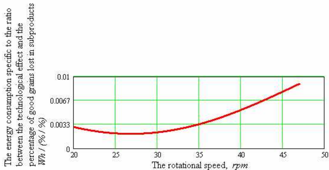
Figure 5: The variation of energy consumption specific to the ratio between the technological effect and the percentage of good grains lost in subproducts, depending on the rotation speed of indented cylinder
