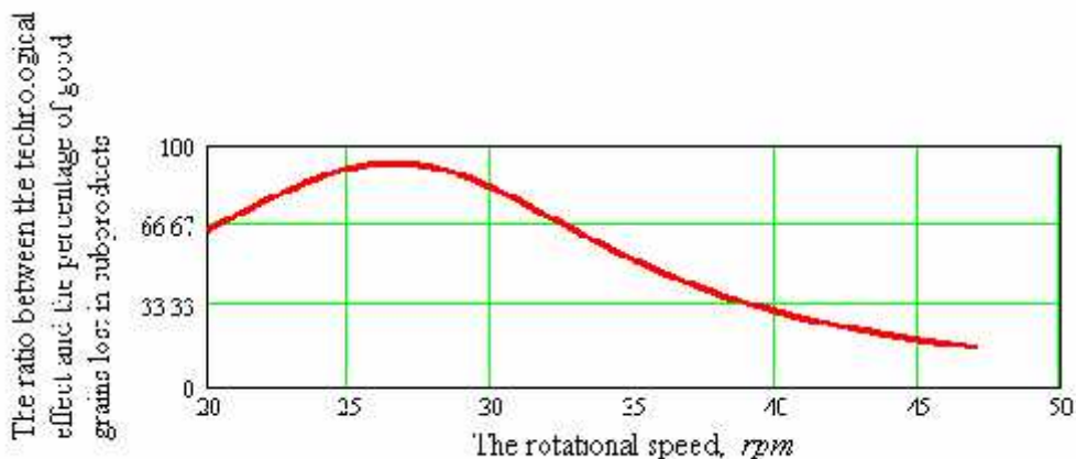
Figure 4: The variation of the ratio between the technological effect and the percentage of good grains lost in subproducts, depending on the rotation speed of the indented cylinder
