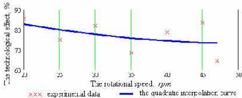
Figure 1: The variation of technological effect depending on the rotation speed of the indented cylinder
