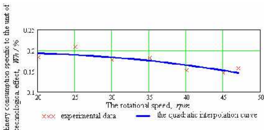
Figure 2: The variation of energy consumption specific to the unit of technological effect depending on the rotation speed of the indented cylinder separator
