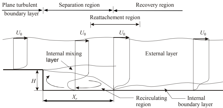
Figure 1: Flow configuration.
