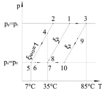
Fig. 5. Thermodynamic cycle of the installation processes in p-\theta-\xi diagram First the pressures are determined:
