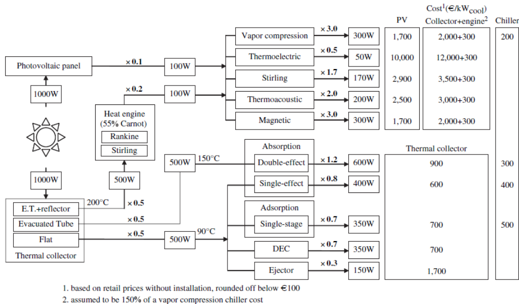
Fig. 2. Cost-efficiency for different solar cooling systems. [9]
