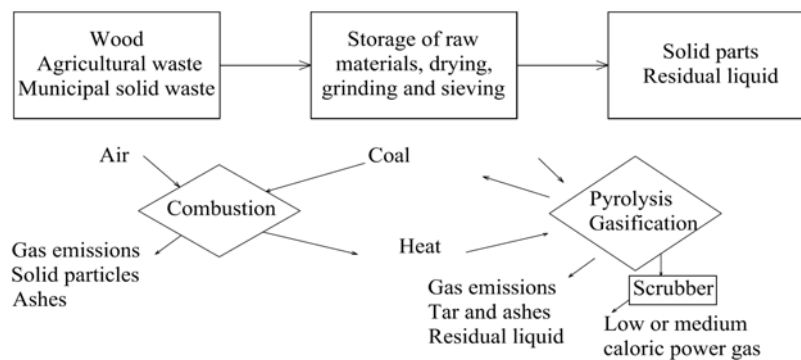
Fig. 3 Combustion processes diagram
