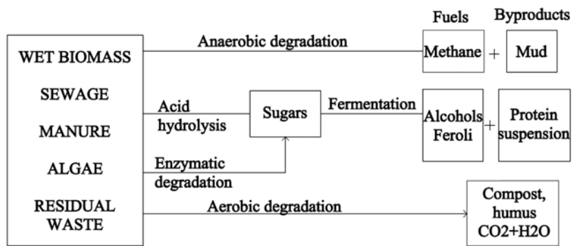
Fig. 2 Wet biomass conversion technologies
