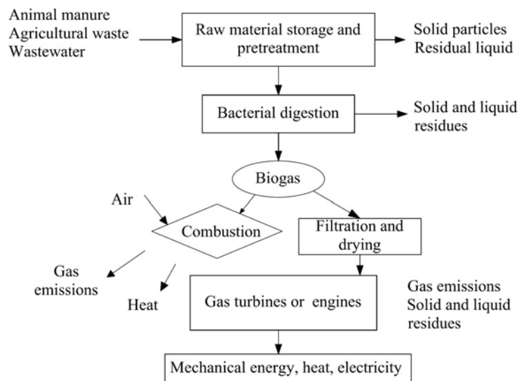
Fig. 5 Diagram of anaerobic digestion process
