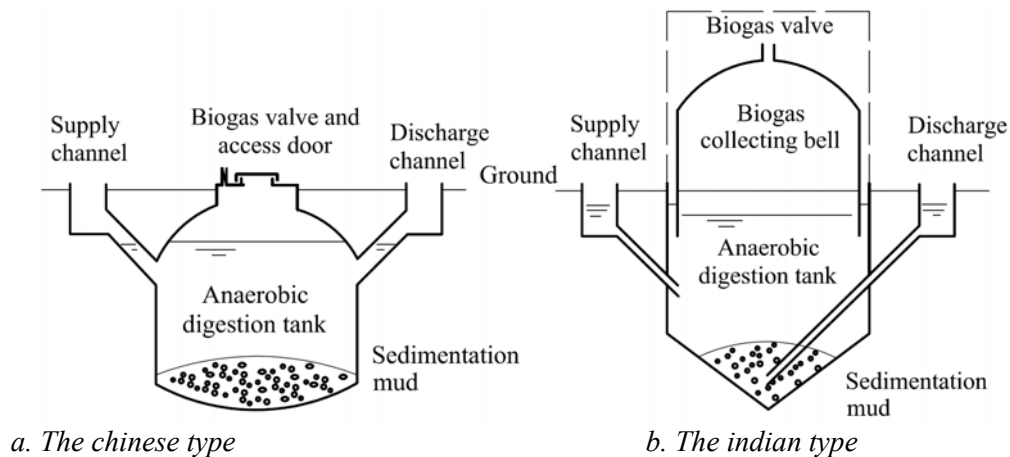
Fig. 6 Types of rural biogas reactors
