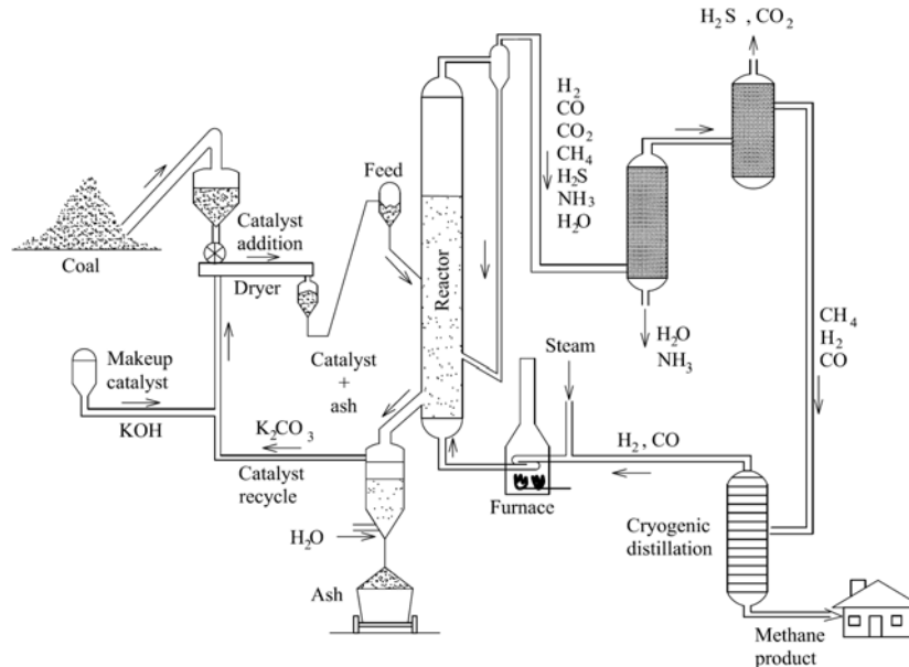
Fig. 4 The scheme of catalytic gasification process
